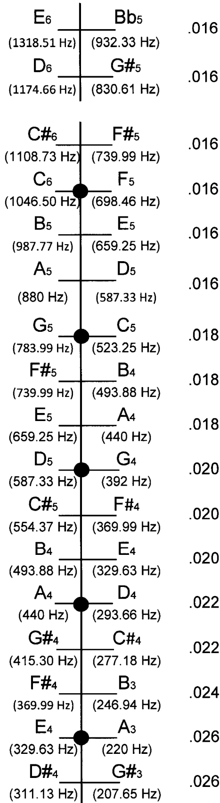
Treble Bridge
